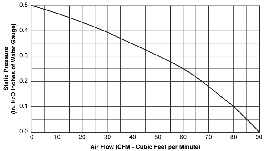
Model AEN80B
