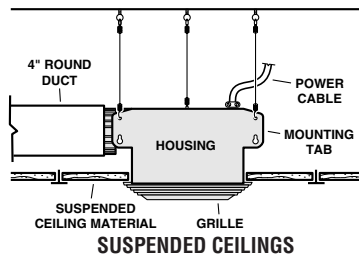
Housing hung with wires - 3-point mount.
