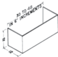
E60000 12" soffit flue cover
